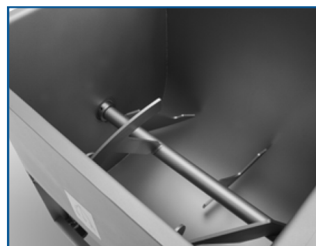
Easily removable mixing shaft with bent shovels and dough-breaking wings
